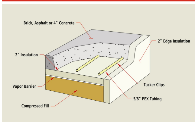
Cross-section of a typical Roth Snow and Ice-Melt System
